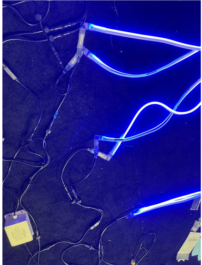
Connections with Dimmer Box
